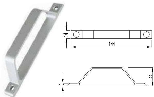
M07-505 D KOL BENT HANDLE D TYPE
