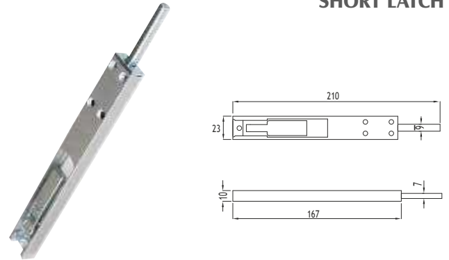
M08-502 KISA GENİŞ SÜRGÜ ( ALDOKS C 60 ) SHORT LATCH
