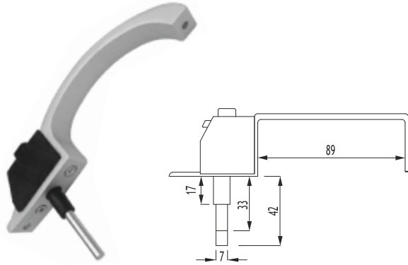
M07-503 TETİK KOL SLIDING HANDLE
